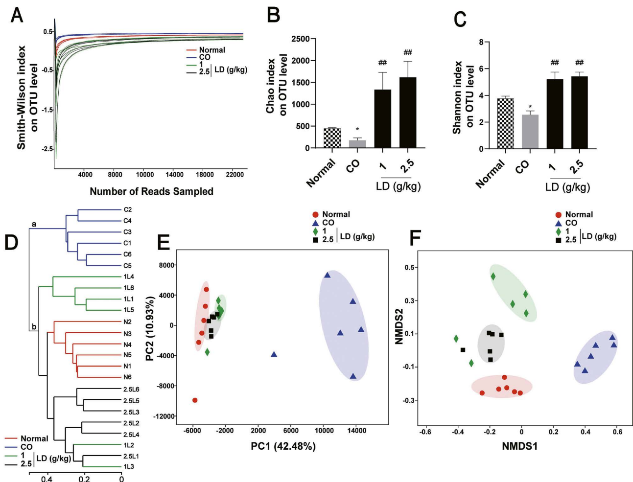
Fig. 3. Effects of LD on the general composition of gut microbiota in mice with CO-induced diarrhoea. (A) Smith Wilson rarefaction curves on the OTU level of gut microbiota in mice with diarrhoea. Alpha diversity of gut microbiota in mice with diarrhoea is shown via (B) Chao and (C) Shannon indices on the OTU level. Beta diversity of gut microbiota in mice with diarrhoea is shown via (D) HCA, (E) PCA and (F) NMDS. Data are expressed as means \pm SD, N = 6. *P < 0.05 vs normal group, ##P < 0.01 vs CO group.
