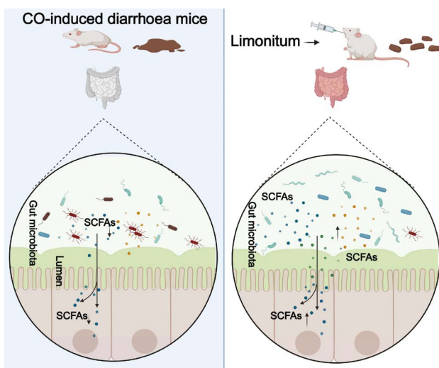
Fig. 6. Schematic diagram of Limonitum-regulated gut microbiota in mice with CO-induced diarrhoea.
