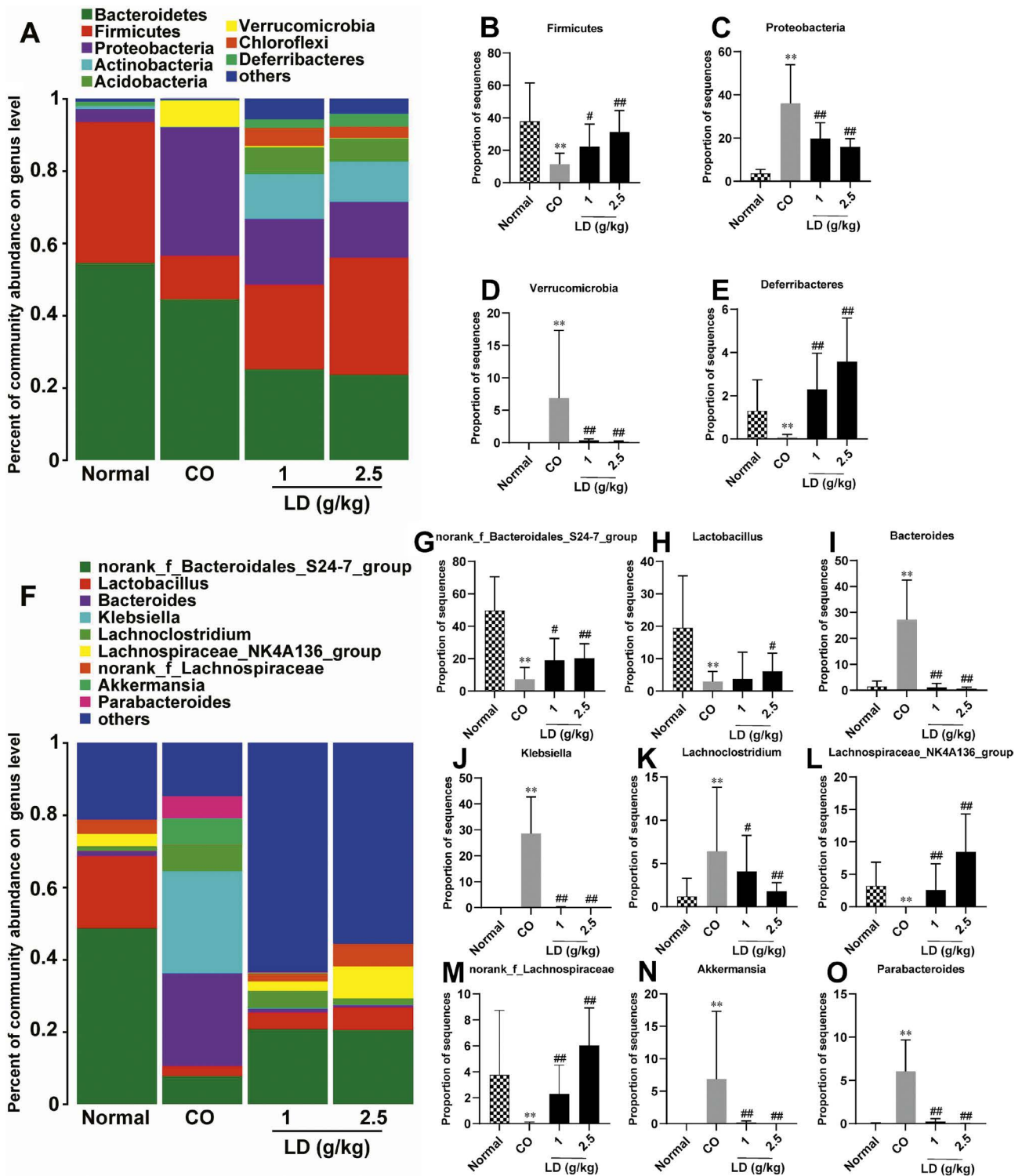
Fig. 4. Effects of LD on the abundance of gut microbiota in mice with CO-induced diarrhoea. (A) Relative abundances of species at the phylum level, including (B) Firmicutes, (C) Proteobacteria, (D) Verrucomicrobia and (E) Deferribacteres. (F) Relative abundances of species at the genus level, including (G) norank_f_Bacteroidales_S24-7_group , (H) Lactobacillus , (I) Bacteroides , (J) Klebsiella , (K) Lachnoclostridium , (L) Lachnospiraceae_NK4A136_group , (M) norank_f_Lachnospiraceae , (N) Akkermansia and (O) Parabacteroides . Data are expressed as means \pm SD, N = 6. **P < 0.01 vs normal group, #P < 0.05 and ##P < 0.01 vs CO group.
