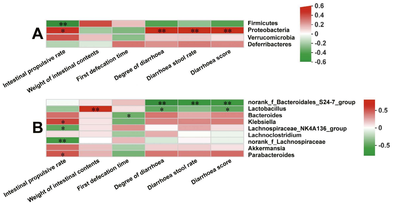
Fig. 5. Pearson's correlation analysis between diarrhoea symptoms and species. (A) Phylum. (B) Genus. * P < 0.05 and ** P < 0.01 .
